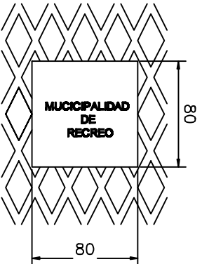
DETALLE "D"
